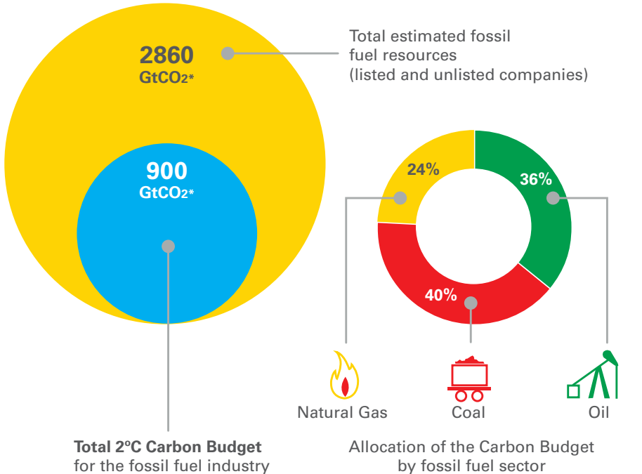
Figure 4: A 'Carbon Budget' maintain just a 2°C temperature increase
